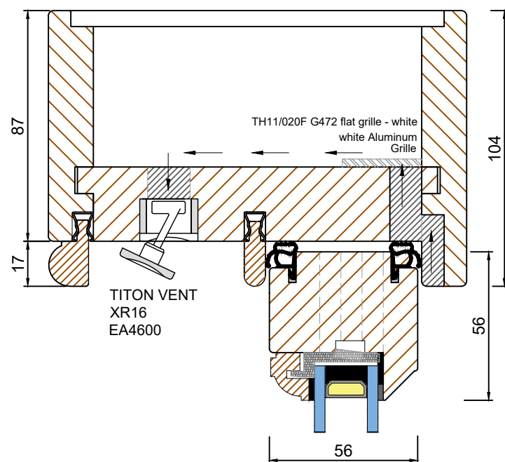
TRICKLE VENT CONCEALED (Scale 1:2)
