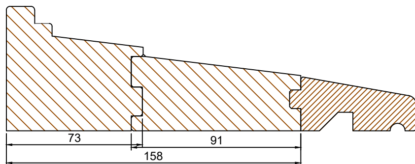
CILL EXTENSION OPTIONS (Scale 1:2)
