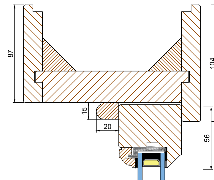
Curved head with fixed sash D-D (Scale 1:2)
