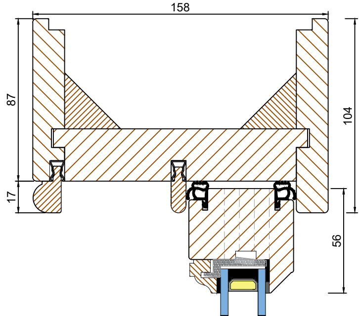
LAMBS TONGUE BEAD OPTION (Scale 1:2)
