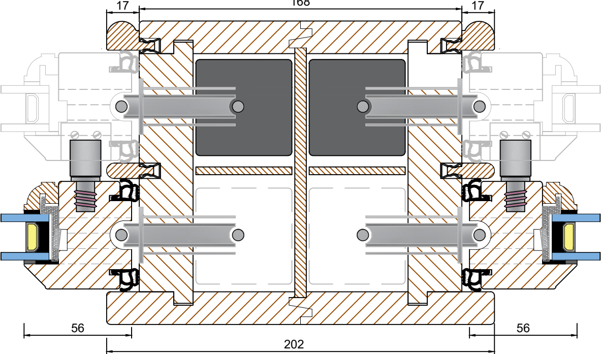
DOUBLE SASH VIEWED EXTERNALLY (Scale 1:10)
