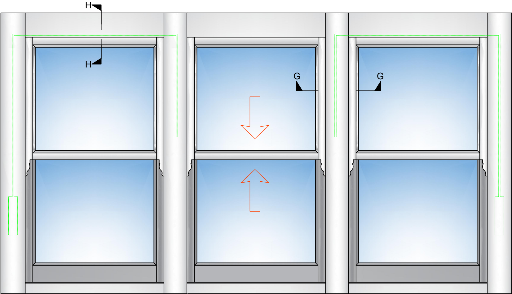
VENETIAN TRIPLE SASH VIEWED EXTERNALLY (Scale 1:10)
