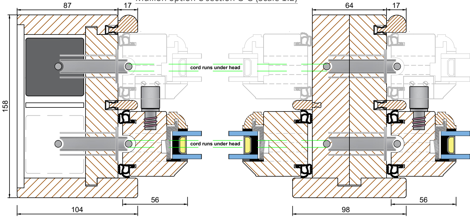
Mullion option C section G-G (Scale 1:2)
