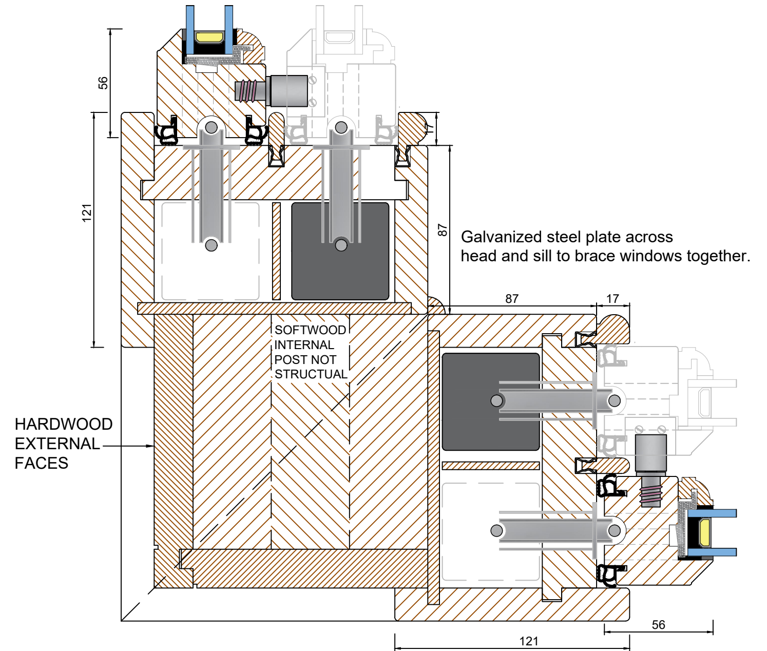
90° Corner Post Option (Scale 1:2)
