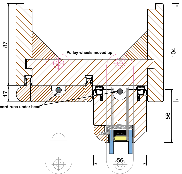
Mullion option C section Through Head H-H (Scale 1:2)
