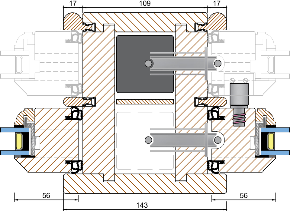
TRIPLE SASH VIEWED EXTERNALLY (Scale 1:10)
