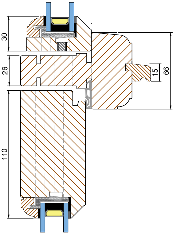
SLIM GLAZED FANLIGHT
