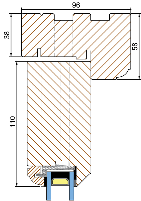
FIXED SIDELIGHT OPTION B (Scale 1:2) HEAD & CILL SECTION C-C
