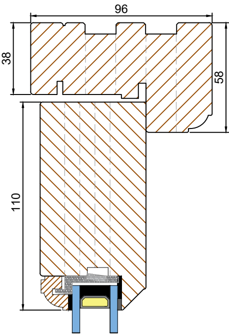
FIXED SIDELIGHT OPTION B (Scale 1:2) HEAD & CILL SECTION E-E
