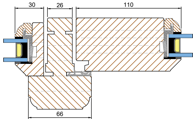
FIXED SIDELIGHT OPTION A (Scale 1:2) BACK TO BACK JAMB
