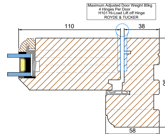
Section E-E - Muntin Rail Options
