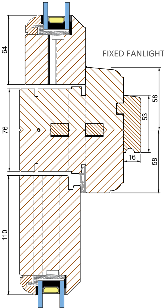
HEAD & CILL LINK WITH OVER DRIP (Scale 1:2)
