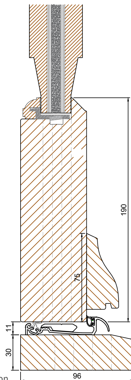
Section B-B - Head and cill
