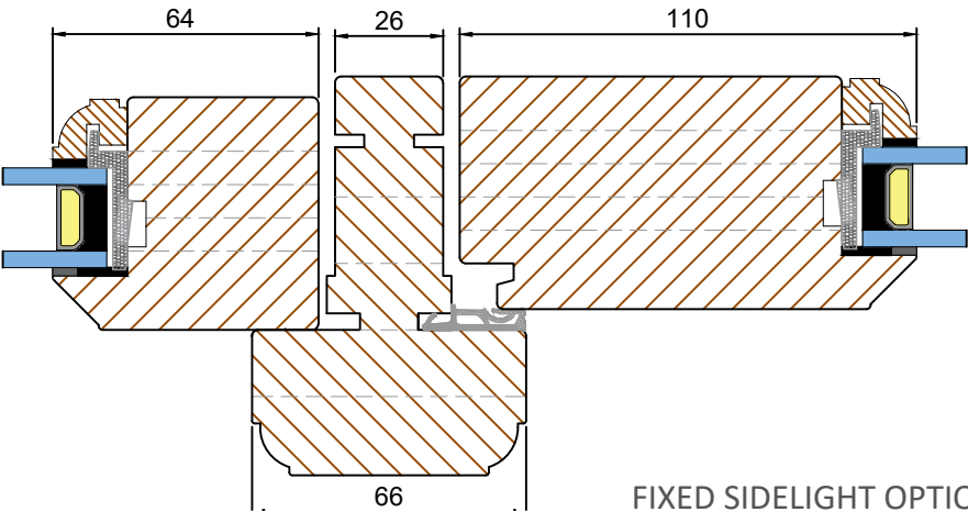
FIXED SIDELIGHT OPTION A (Scale 1:2) BACK TO BACK JAMB
