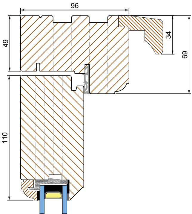
FRAME HEAD DRIP (Scale 1:2)
