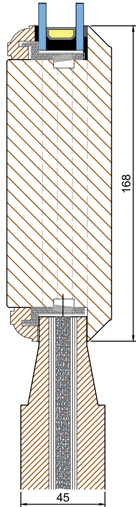
168mm Mid Rail Option (Scale 1:2)
