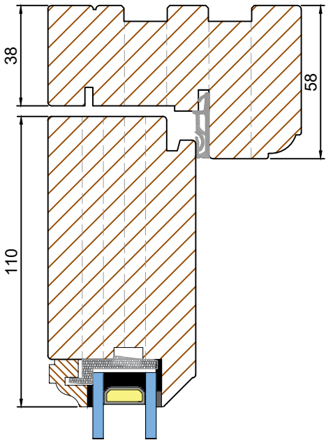
LAMBS TONGUE BEAD OPTION (Scale 1:2)
