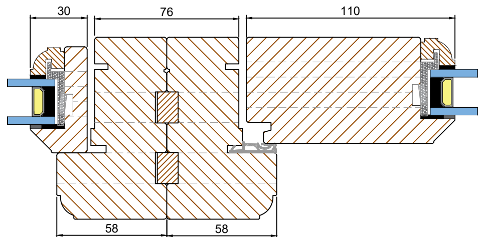
FIXED SIDELIGHT OPTION A (Scale 1:2) BACK TO BACK JAMB
