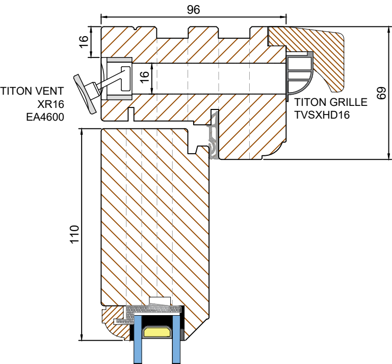
TRICKLE VENT WITH HEAD DRIP (Scale 1:2)
