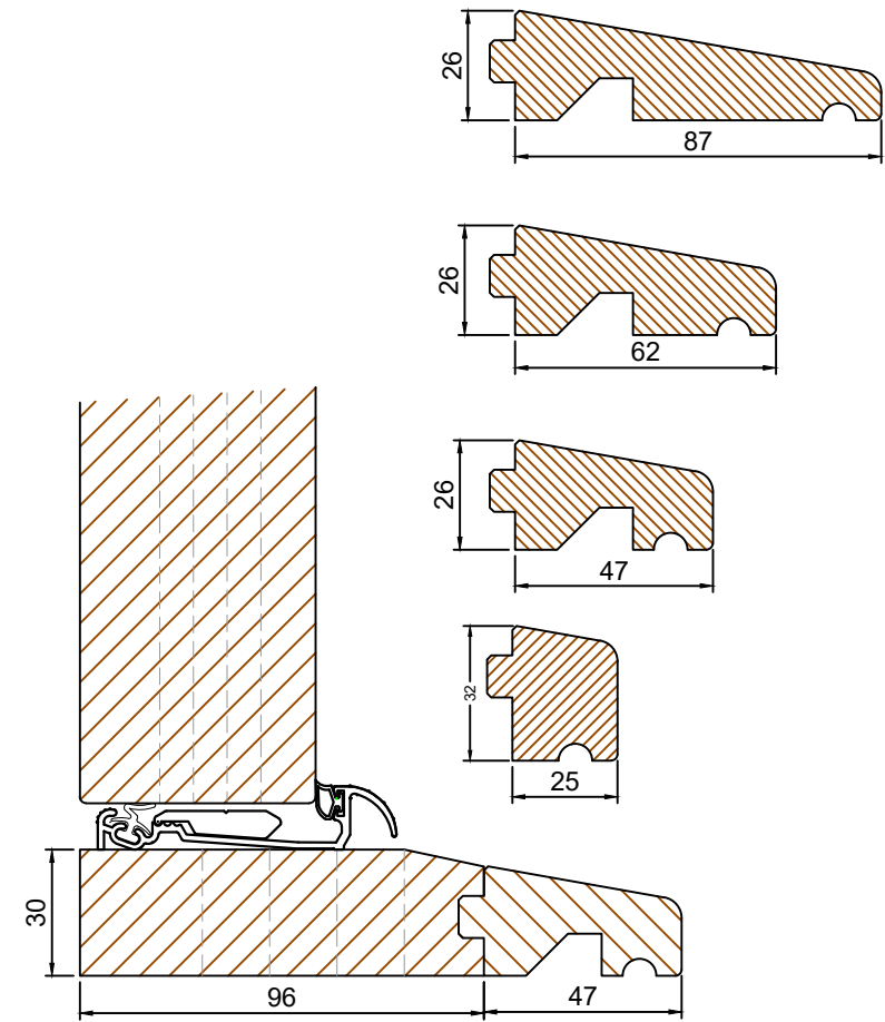
CILL EXTENSION OPTIONS (Scale 1:2)
