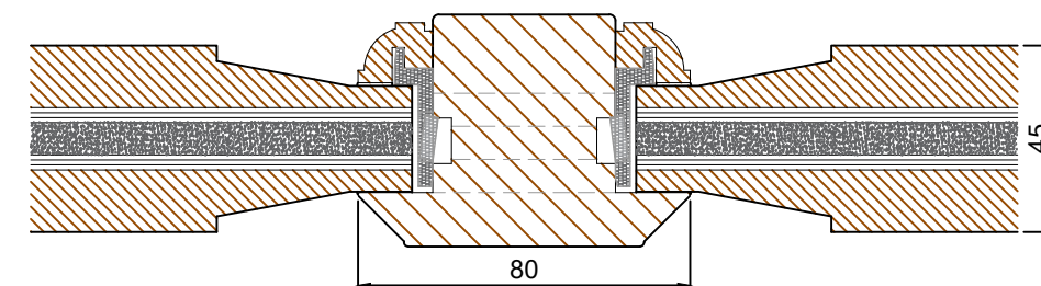
Section E-E - Muntin Rail Options
