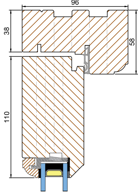
168mm Bottom Rail Option (Scale 1:2) HEAD & CILL
