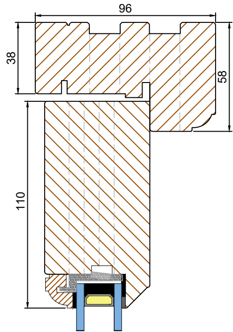
FIXED SIDELIGHT OPTION B (Scale 1:2) HEAD & CILL FULL GLAZED
