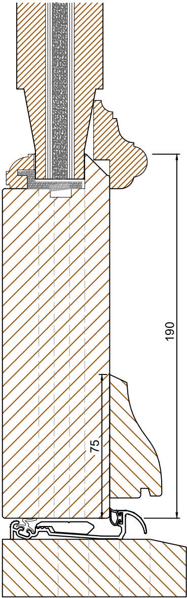
PANEL WITH EXTERNAL BOLECTION MOULD (Scale 1:2)
