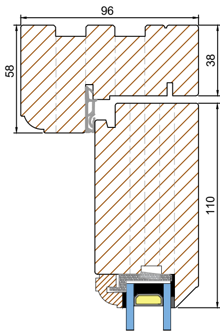
168mm Bottom Rail Option (Scale 1:2) Mobility cill
