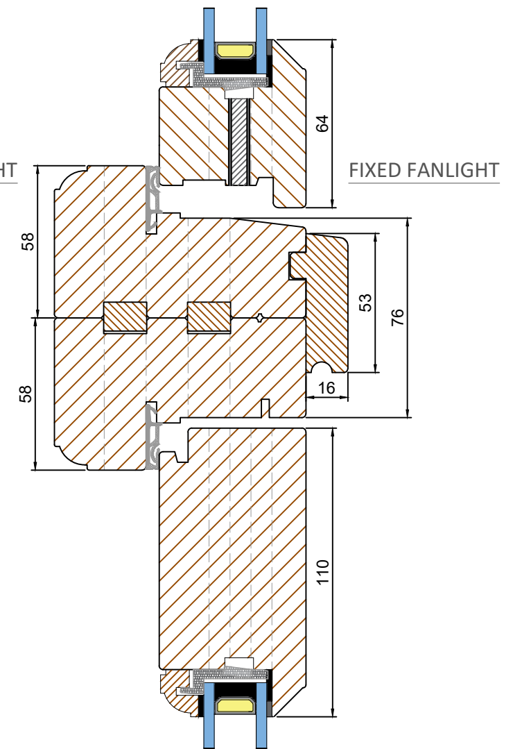
HEAD & CILL LINK WITH OVER DRIP (Scale 1:2)
