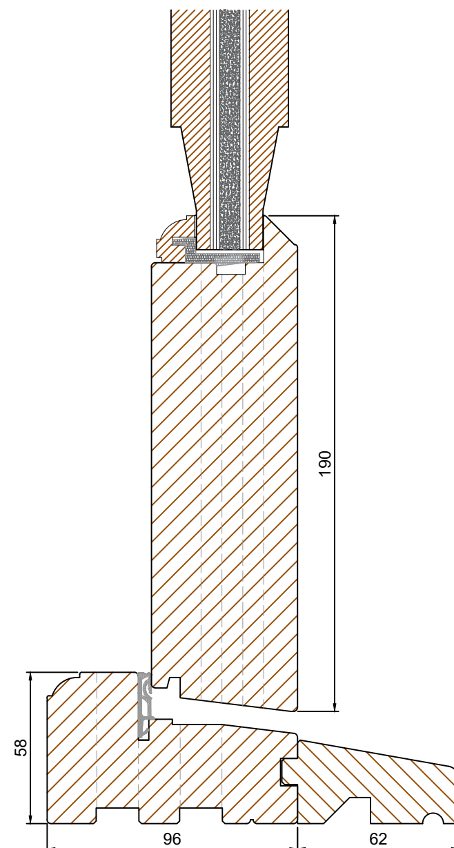
Section B-B - Head and cill
