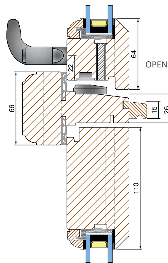
TRANSOM OPTION + DRIP (Scale 1:2)
