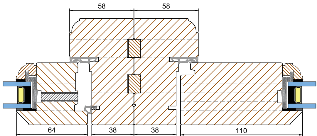
FIXED SIDELIGHT OPTION A (Scale 1:2) BACK TO BACK JAMB
