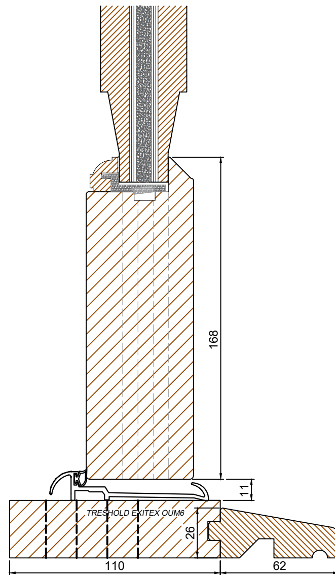
168mm Bottom Rail Option (Scale 1:2) Mobility cill
