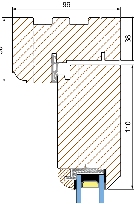
STABLE DOORSET (Scale 1:2) HEAD & CILL
