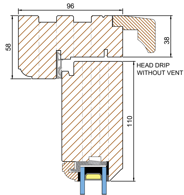
FRAME HEAD DRIP (Scale 1:2)
