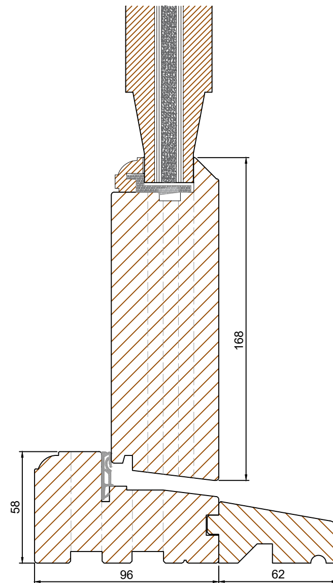
168mm Bottom Rail Option (Scale 1:2) Standard open out cill
