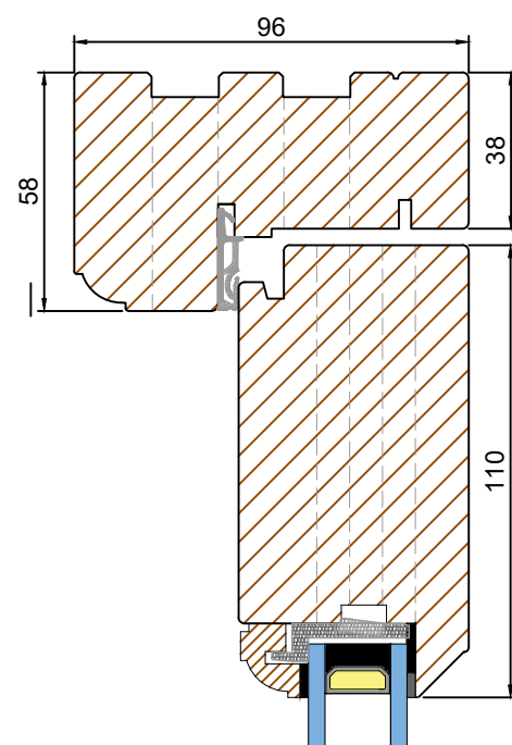
Section B-B - Head and cill
