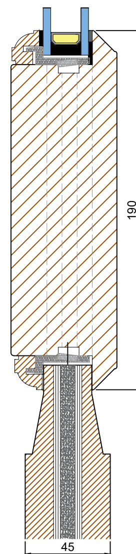
Section C-C - Mid Rail
