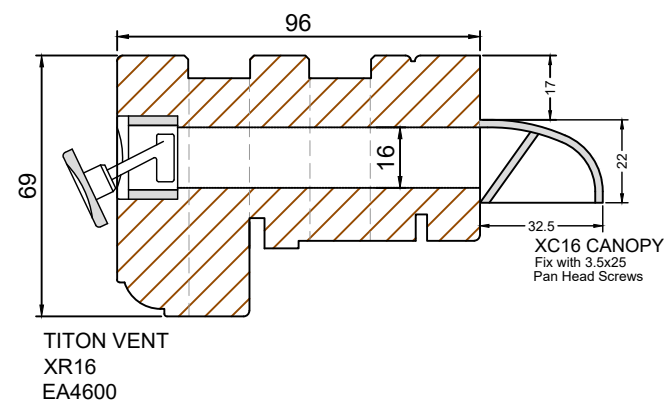
TRICKLE VENT WITH CANOPY (Scale 1:2)
