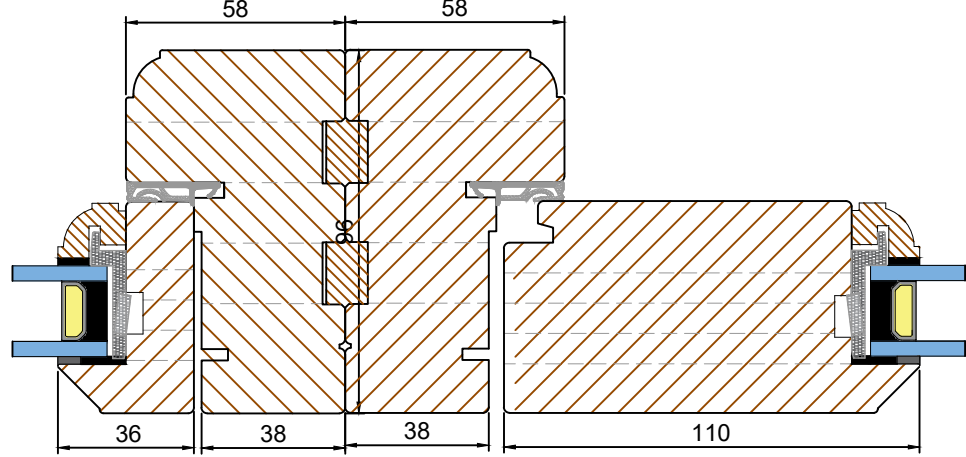
FIXED SIDELIGHT OPTION A (Scale 1:2) BACK TO BACK JAMB
