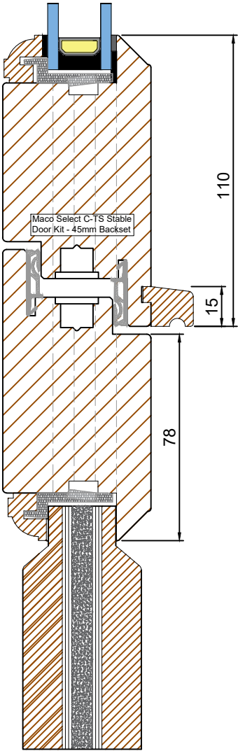
STABLE DOORSET (Scale 1:2) JAMBS & MEETING RAILS SECTION J - J
