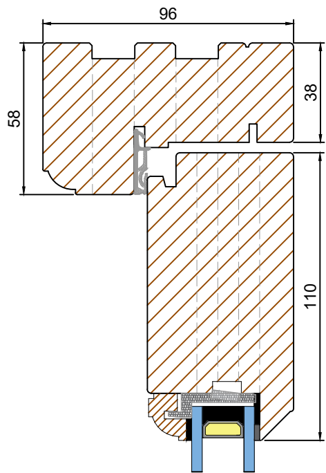
FIXED SIDELIGHT OPTION B (Scale 1:2) HEAD & CILL SECTION E-E
