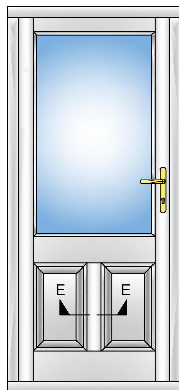
ELEVATIONS (Scale 1:20) Elevation 2 - Inside View
