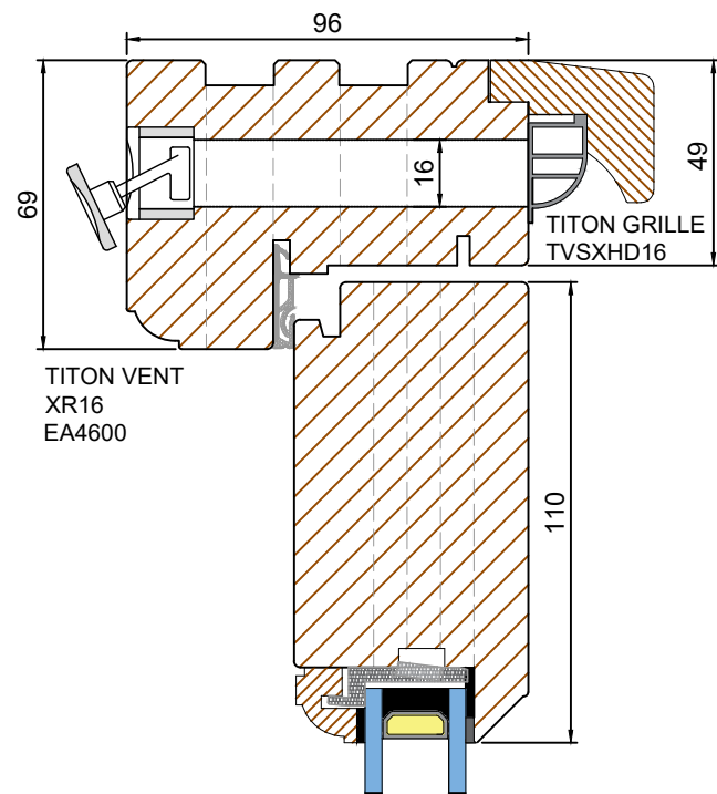
TRICKLE VENT WITH HEAD DRIP (Scale 1:2)
