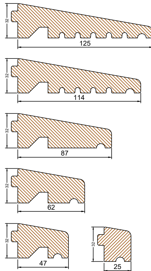
CILL EXTENSION OPTIONS (Scale 1:2)
