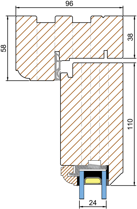
FIXED SIDELIGHT OPTION B (Scale 1:2) HEAD & CILL FULL GLAZED
