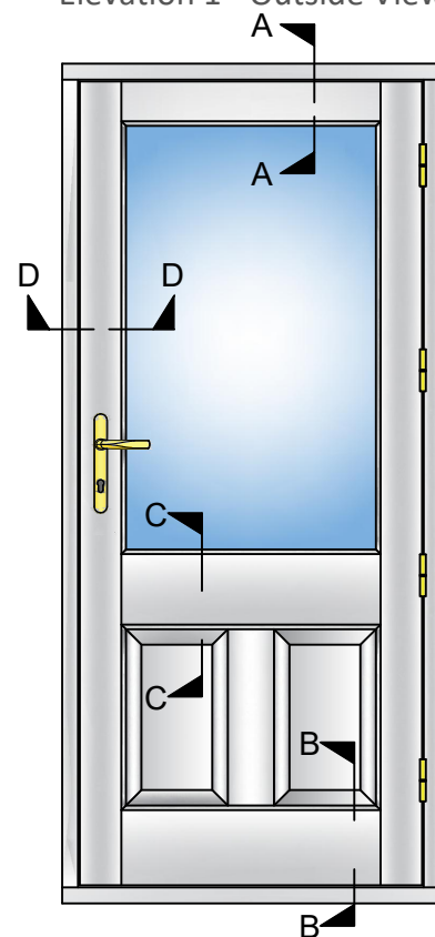
ELEVATIONS (Scale 1:20) Elevation 1 - Outside View
