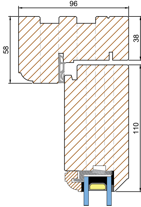
FIXED SIDELIGHT OPTION B (Scale 1:2) HEAD & CILL SECTION C-C
