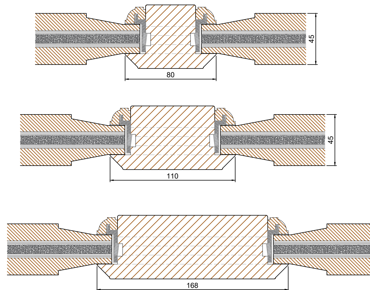
Section E-E - Muntin Rail OPTIONS
