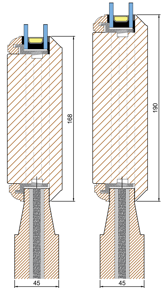
Mid Rail Options (Scale 1:2)
