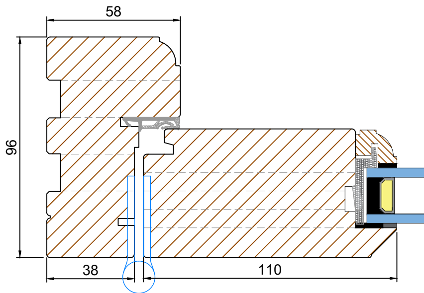
ROYDE & TUCKER H101 Hi-Load Lift off Hinge 4 Hinges Per Door Maximum Adjusted Door Weight 80kg
