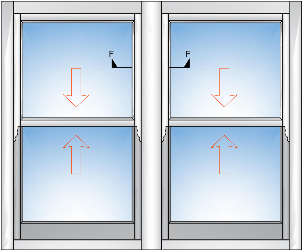
DOUBLE SASH VIEWED EXTERNALLY (Scale 1:10)
