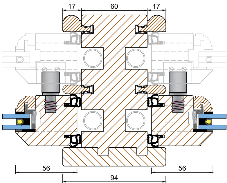
Mullion option B section F-F (Scale 1:2)
