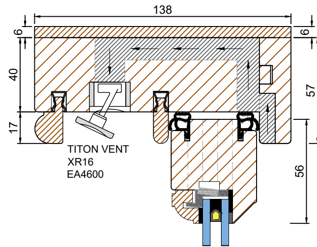
TRICKLE VENT CONCEALED (Scale 1:2)
