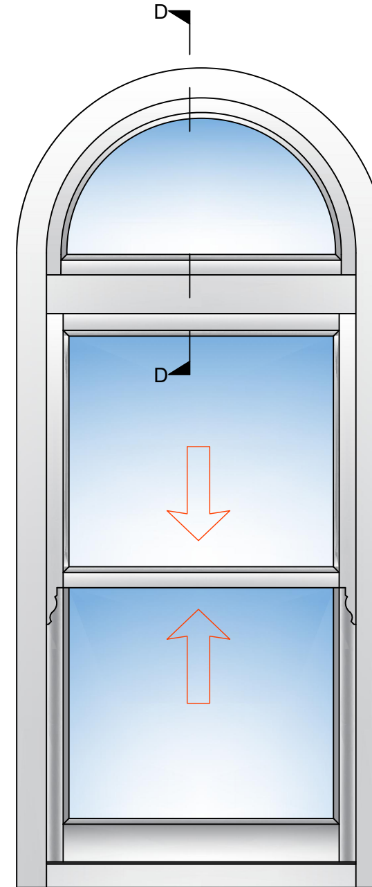
Curved Head Elevation (Scale 1:10)
