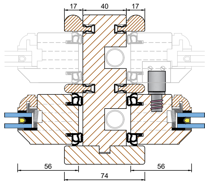
Mullion option A section E-E (Scale 1:2)
