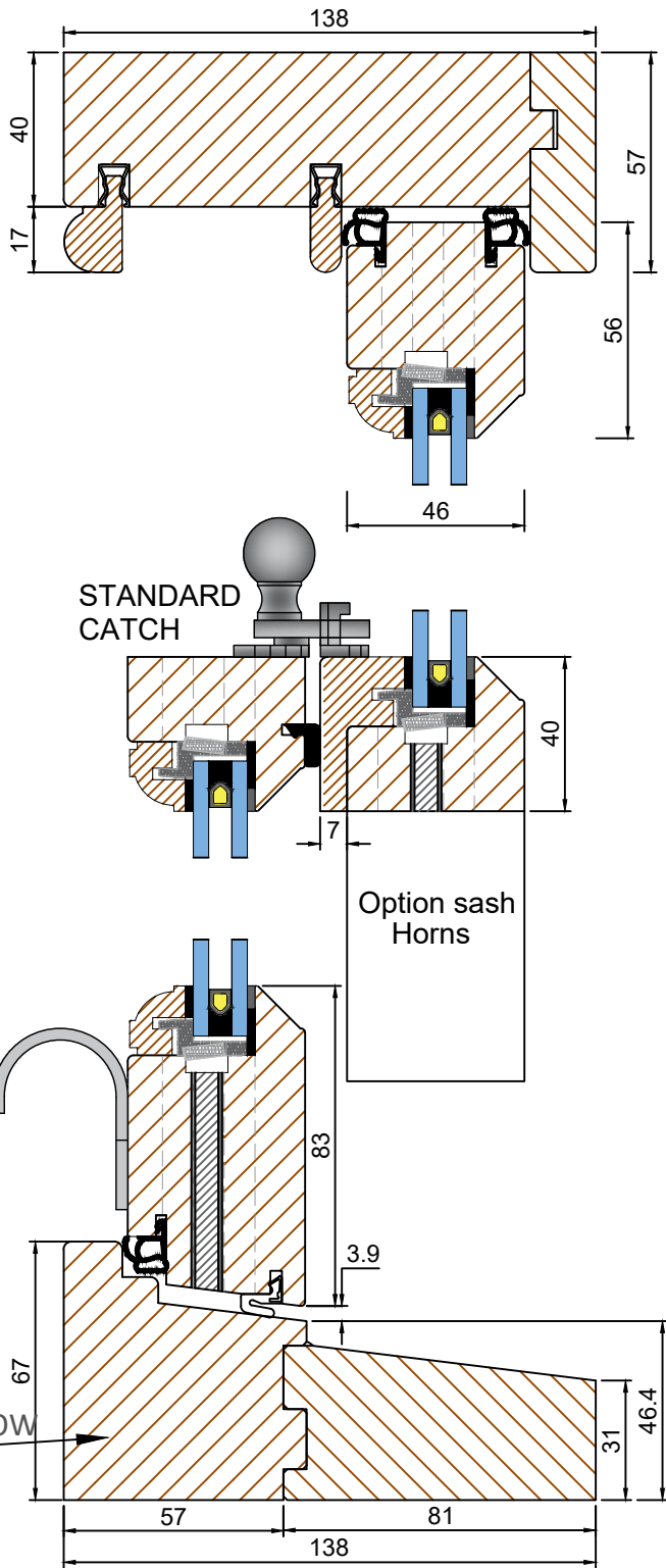
Section B-B - Head and cill
