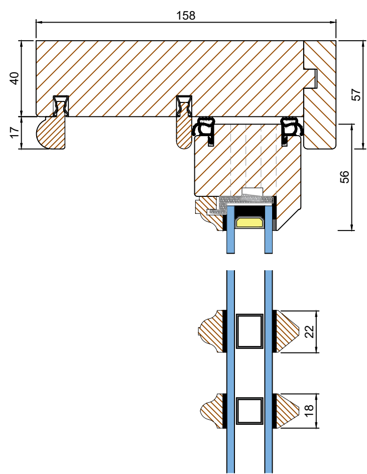
LAMBS TONGUE BEAD OPTION (Scale 1:2)
