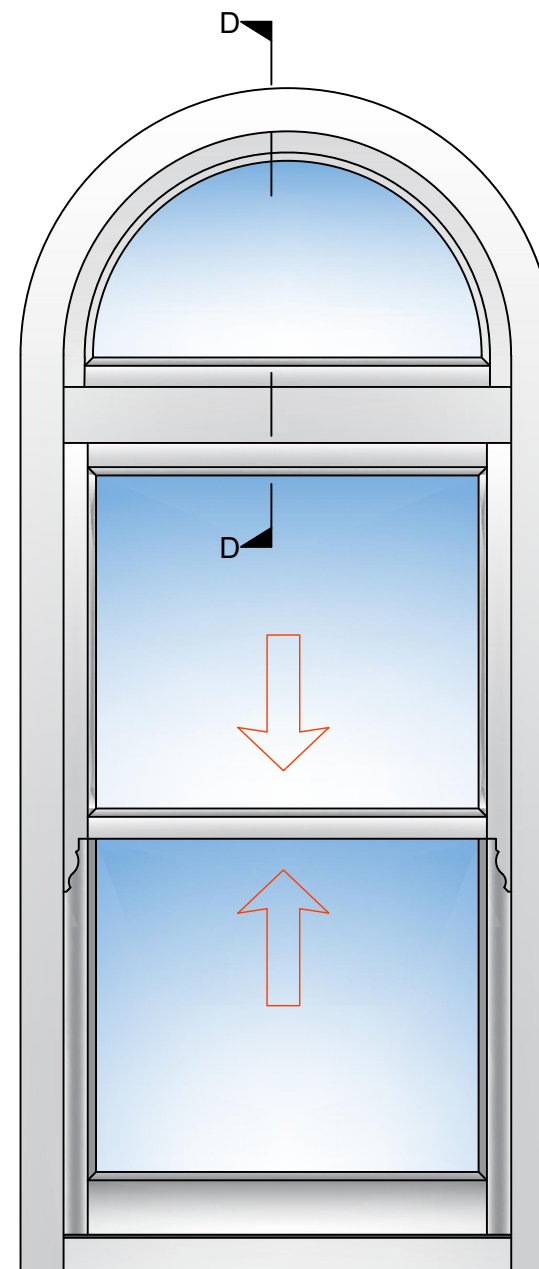
Curved Head Elevation (Scale 1:10)
