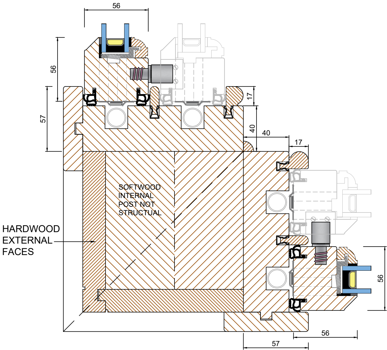
90° Corner Post Option (Scale 1:2)
