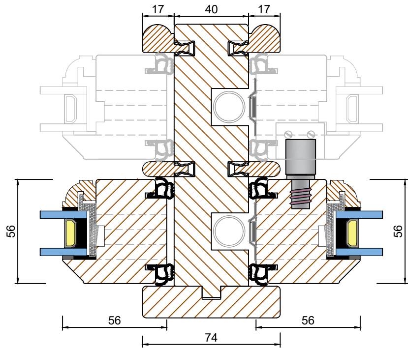
Mullion option A section E-E (Scale 1:2)
