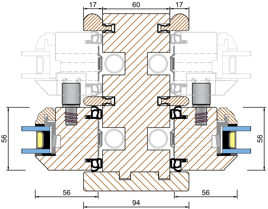
DOUBLE SASH VIEWED EXTERNALLY (Scale 1:10)
